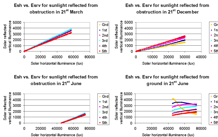
Figure 3: Contribution of the sunlight reflected from obstruction and/or ground to the solar reflected vertical illuminance, Esvr, and the solar horizontal illuminance, Esh, for several floor heights on a north façade for the equinox and solstice days.
